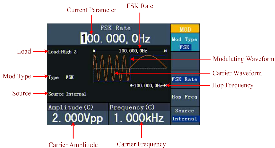
Figure 0-19: The User Interface of FSK
